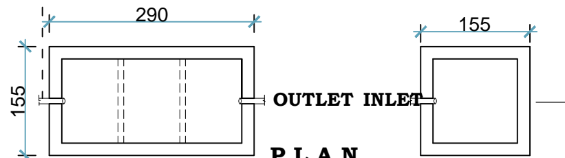
DETAILS OF SEPTIC TANK AND SOAK PIT
